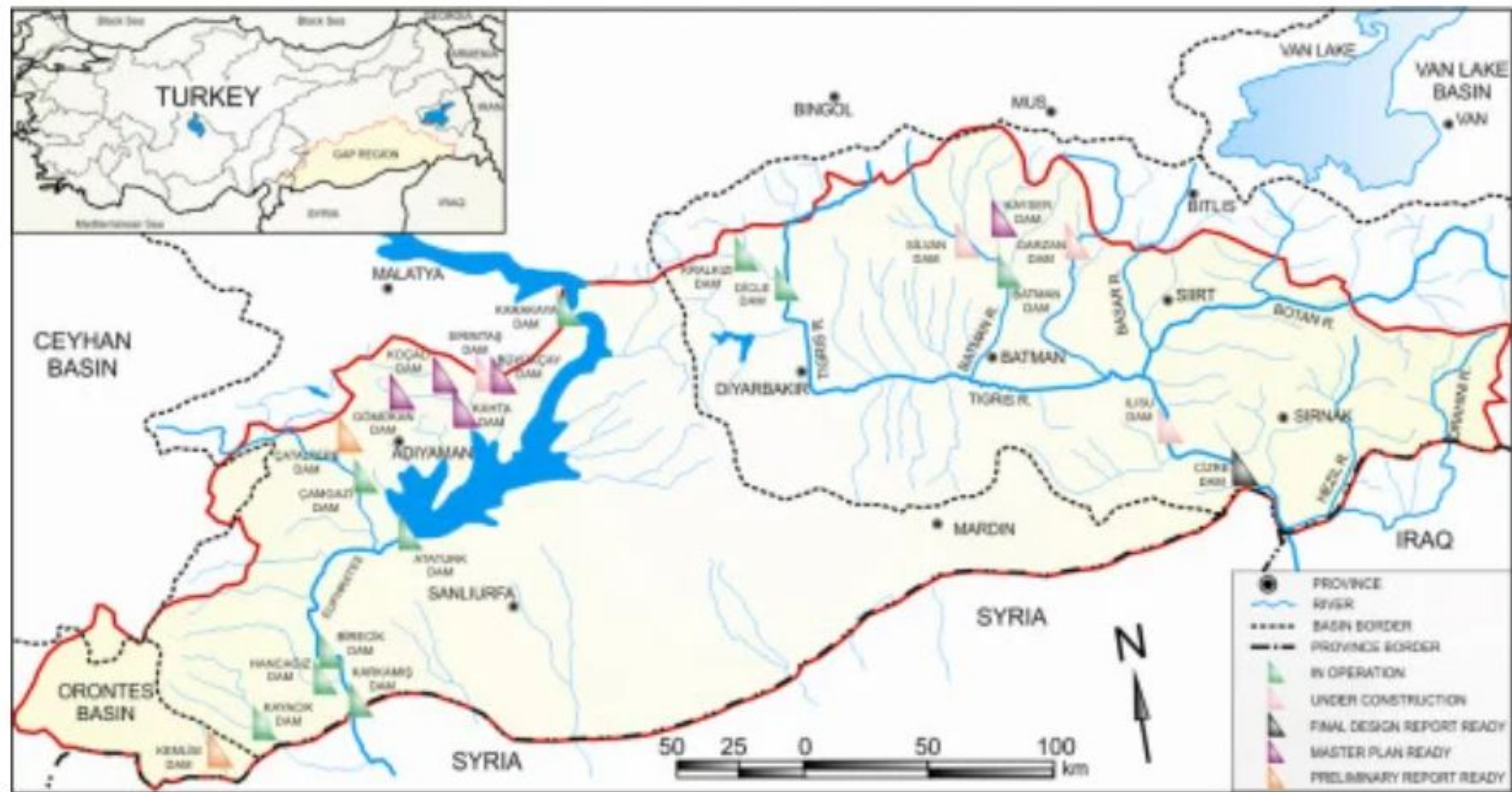
The dams and HEPPs in the GAP (Republic of Turkey, 2013a).
